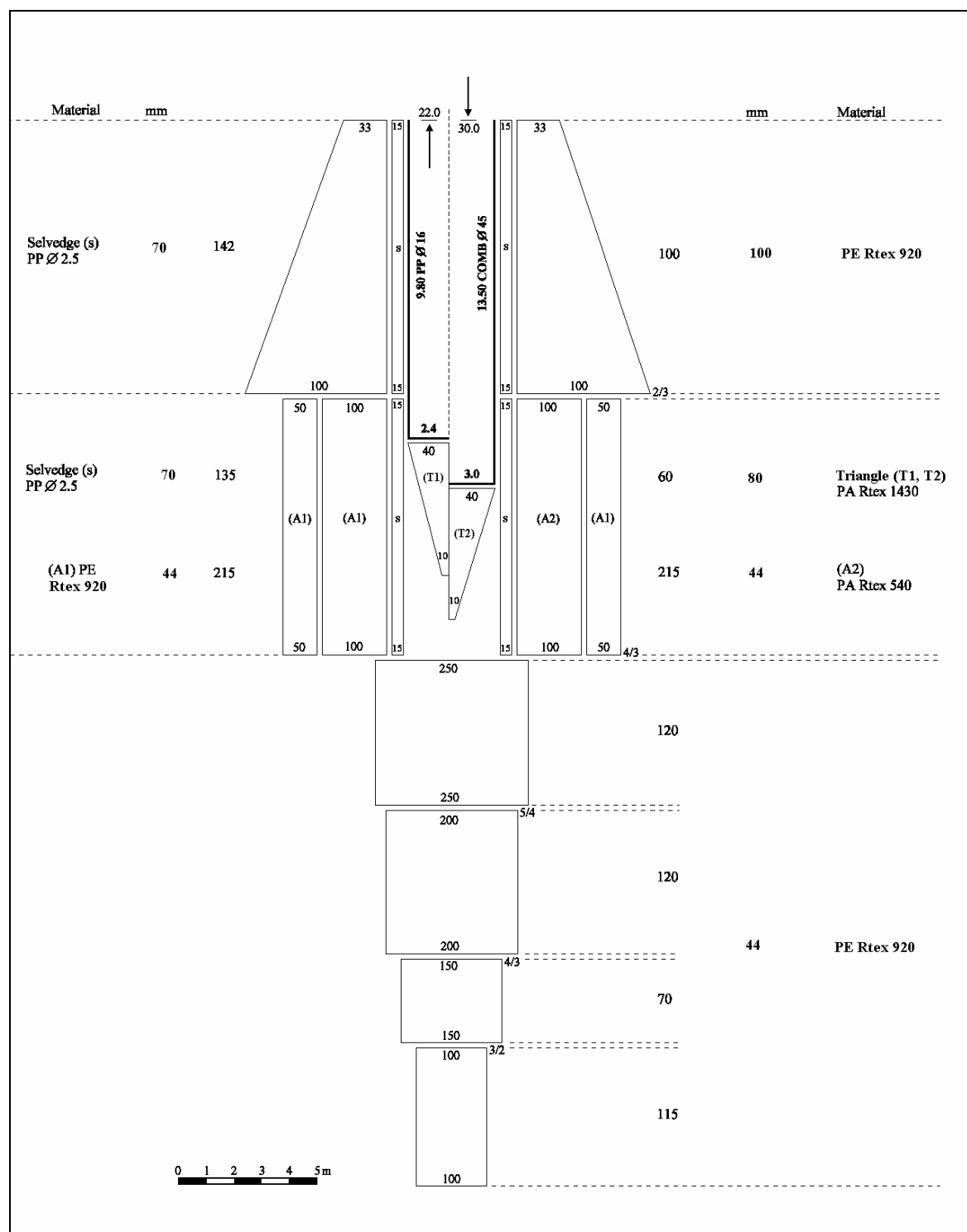
Fig. 2. Commercial bottom trawl net used in sampling (Redrawn from TOSUNOĞLU et al., 1996)
